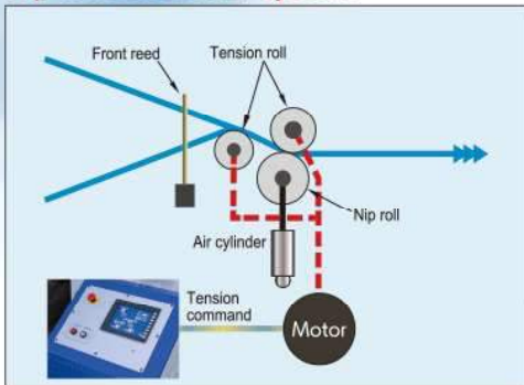
Nip tension control system
